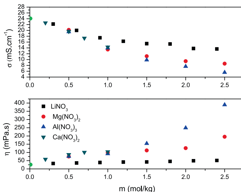
Fig. 7. Concentration dependence of the conductivity (a) and the viscosity (b) for pure EAN and its mixtures with LiNO 3 , Mg(NO 3 ) 2 , Ca(NO 3 ) 2 and Al(NO 3 ) 3 at 298.15 K. Green dots correspond to the values of pure EAN (data taken from Ref. [53]).
